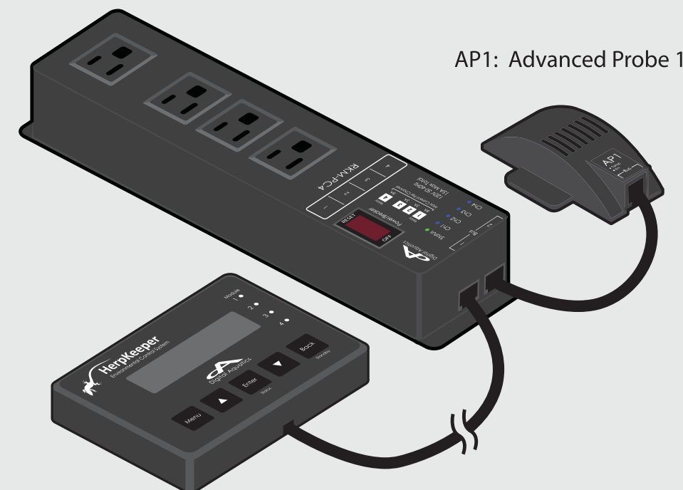
HK PLUS: Connection Example
