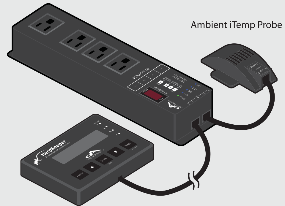
HK BASIC: Connection Example
