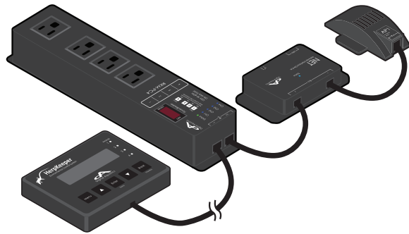
HerpKeeper NET: Connection Example
